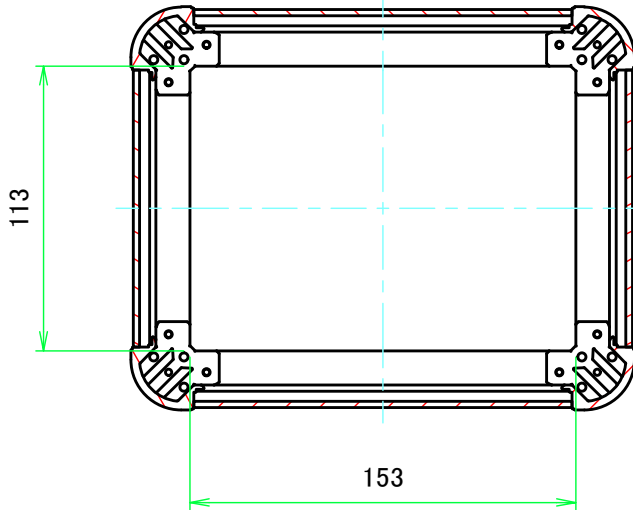
C-C (1:3)
